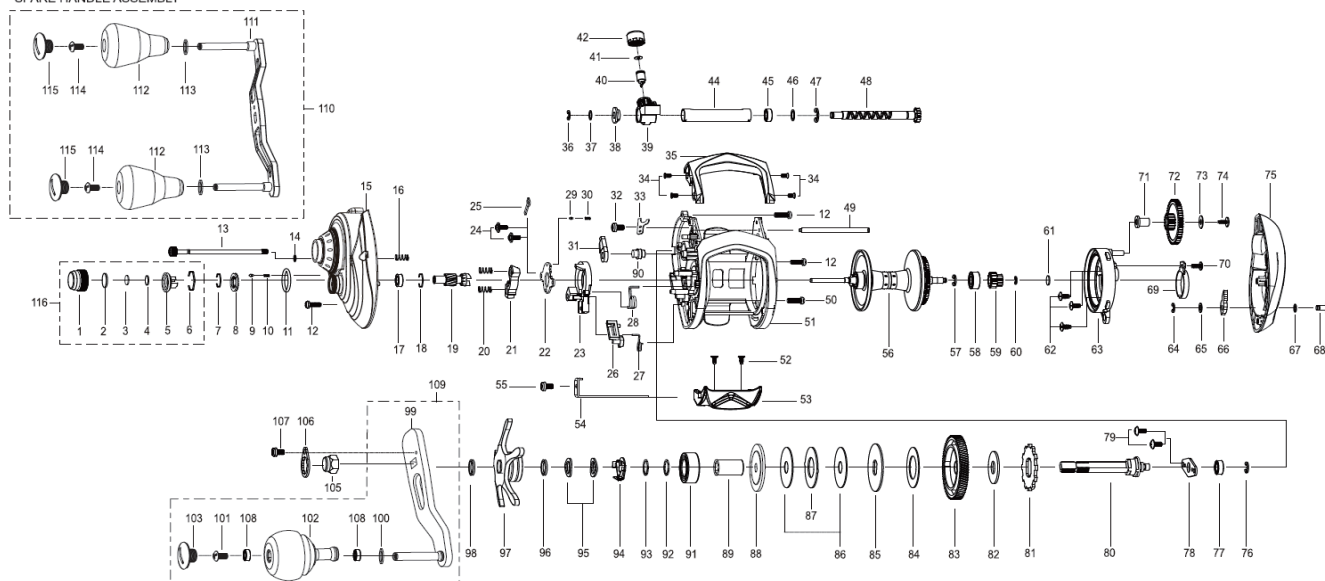
*SPARE HANDLE ASSEMBLY
